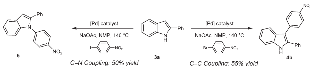
Scheme 3. Dual reactivity in the 2-phenylindole: C–C versus C–N coupling reactions.
