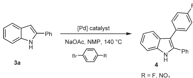
Scheme 2. Cross-coupling arylation at the 3-position of the 2-phenylindole.
