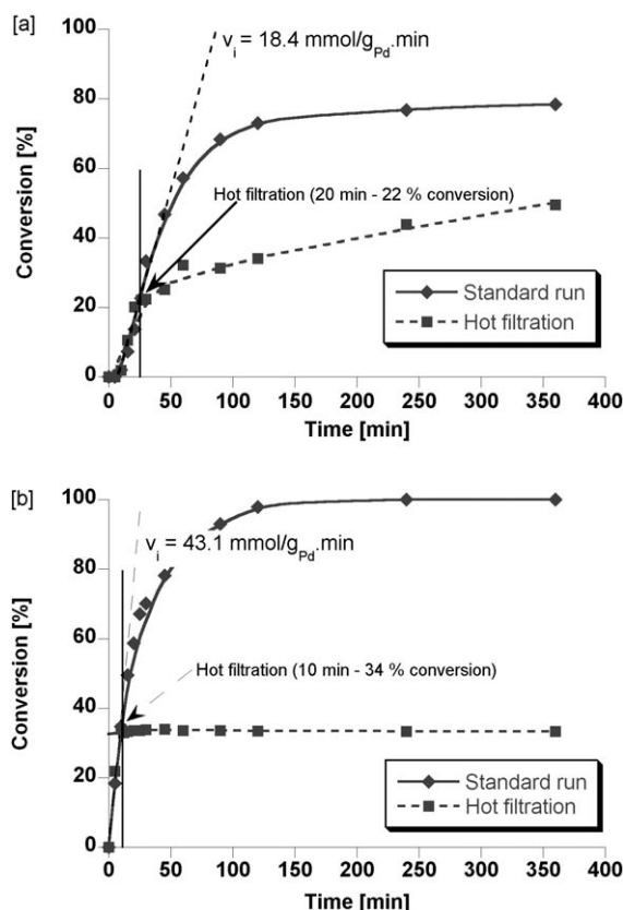
Figure 2. Leaching of active Pd species in solution: [a] using [\text{Pd}(\text{NH}_3)_4]/\text{NaY} and [b] using [\text{Pd}]/\text{SBA-15} catalyst. Reaction conditions: 5 mmol 2-iodoaniline, 7 mmol phenylacetylene, 8 mmol \text{Et}_3\text{N} , 1 mol % [\text{Pd}] catalyst, 10 mL DMF/ \text{H}_2\text{O} (4:1), 80^\circ\text{C} .
