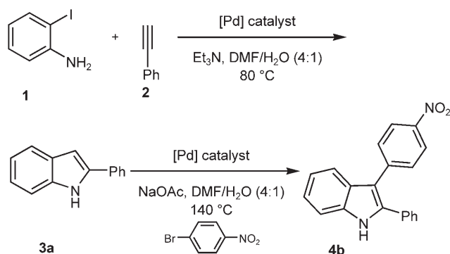
Scheme 5. Direct one-pot synthesis of 2,3-substituted indoles.
