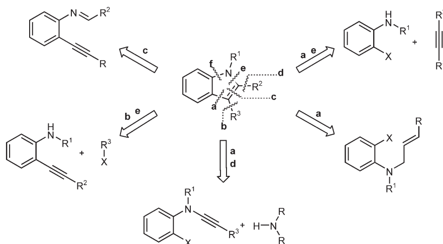
Figure 1. Retro-synthetic approaches toward the synthesis of indole nucleus catalysed by palladium.
